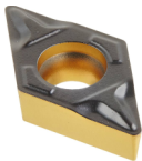
DCMT 070204/08 DCMT 11T304/08
