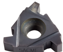
TREADING ACME
